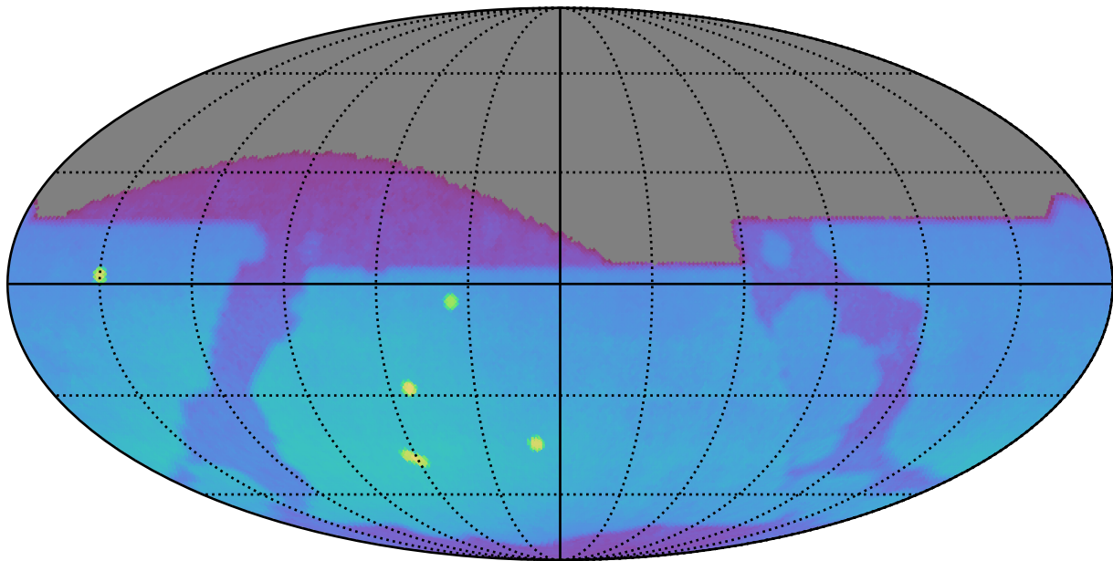
too_combined_s1.5_v3.4_10yrs : Brown Dwarf, L7
