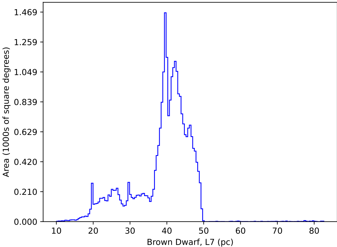
too_combined_s1.5_v3.4_10yrs : Brown Dwarf, L7
