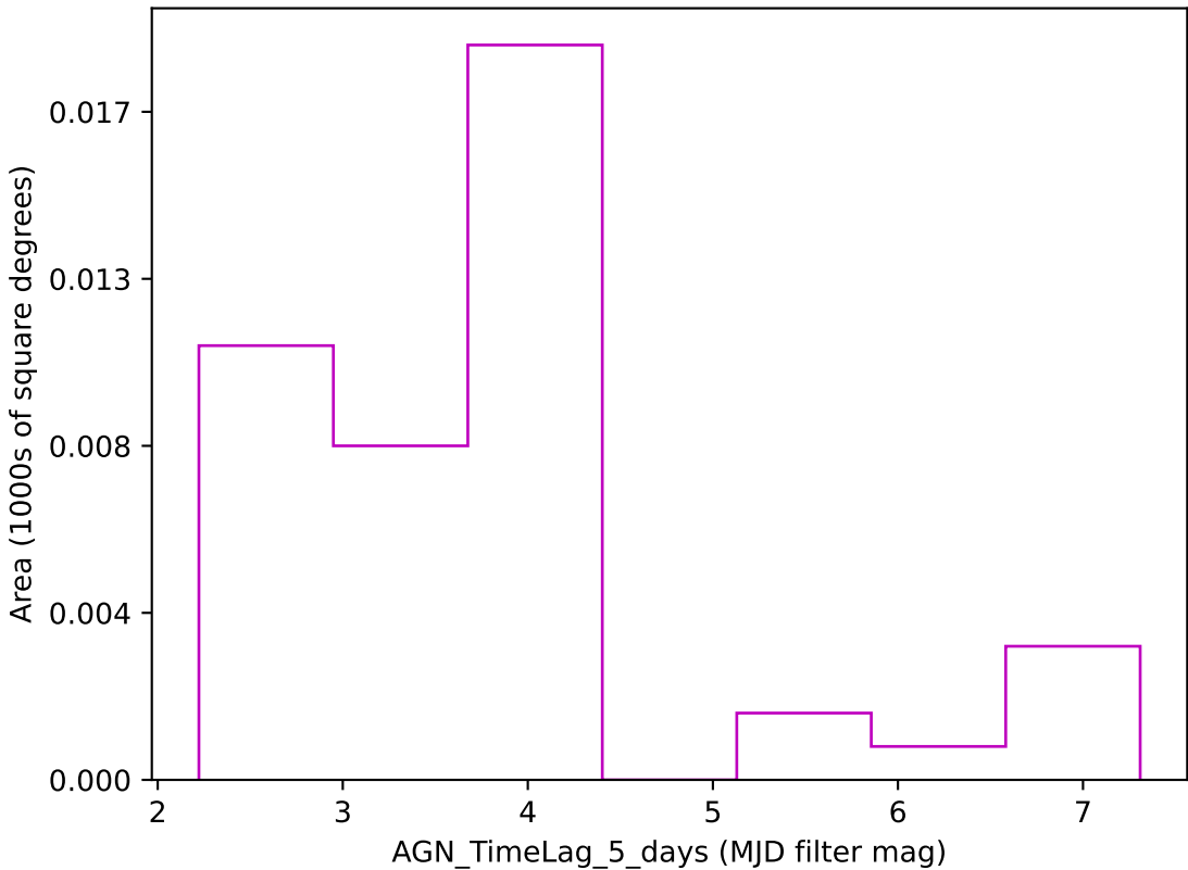
too_combined_s1.5_v3.4_10yrs z band: AGN_TimeLag_5_days
