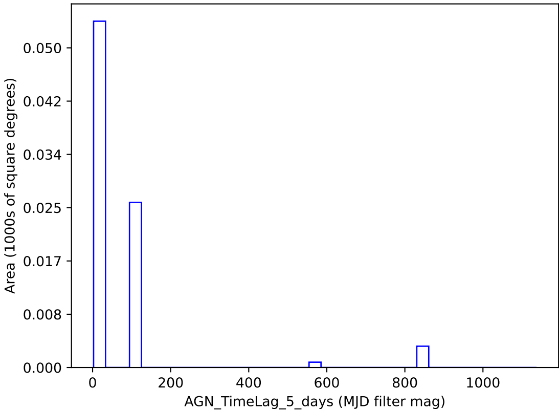
too_combined_s1.5_v3.4_10yrs y band: AGN_TimeLag_5_days
