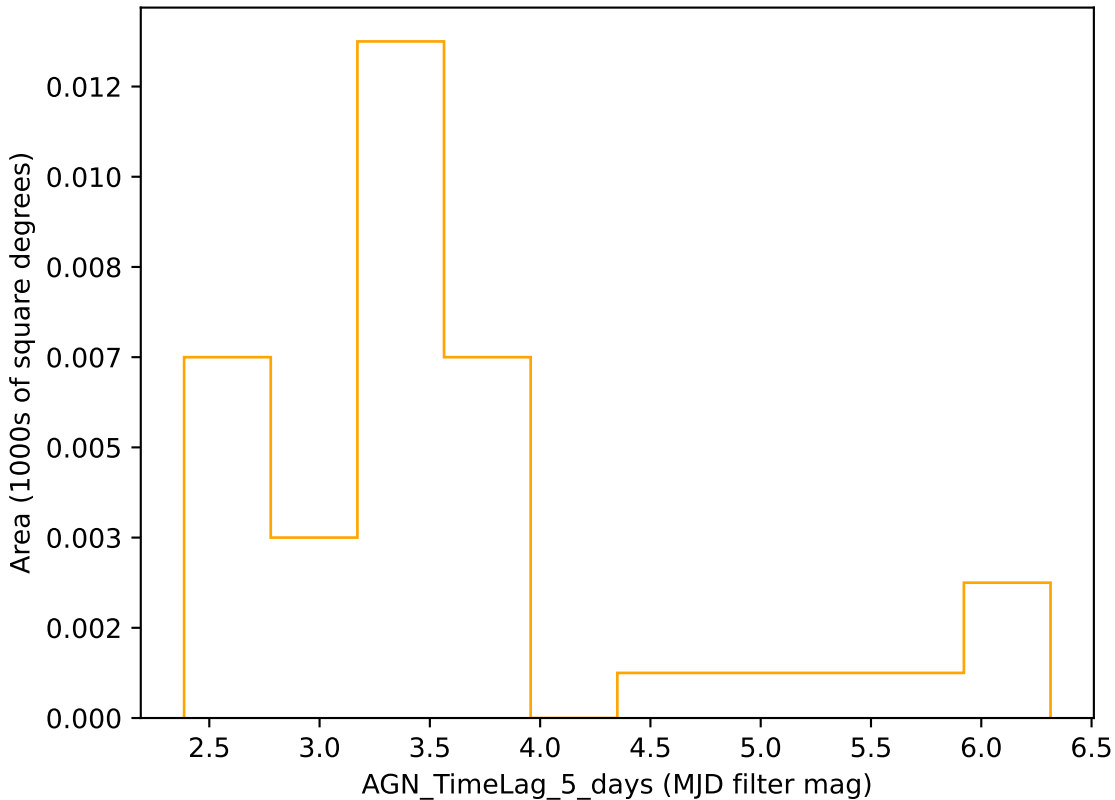
too_combined_s1.5_v3.4_10yrs r band: AGN_TimeLag_5_days
