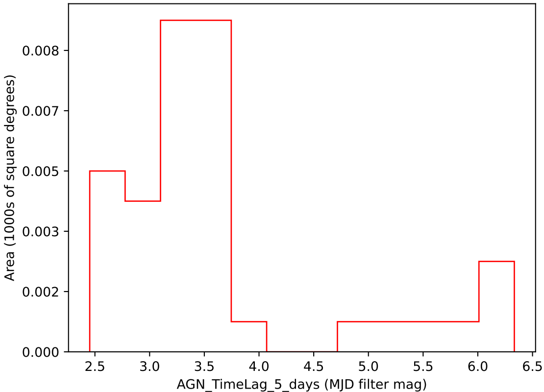
too_combined_s1.5_v3.4_10yrs i band: AGN_TimeLag_5_days
