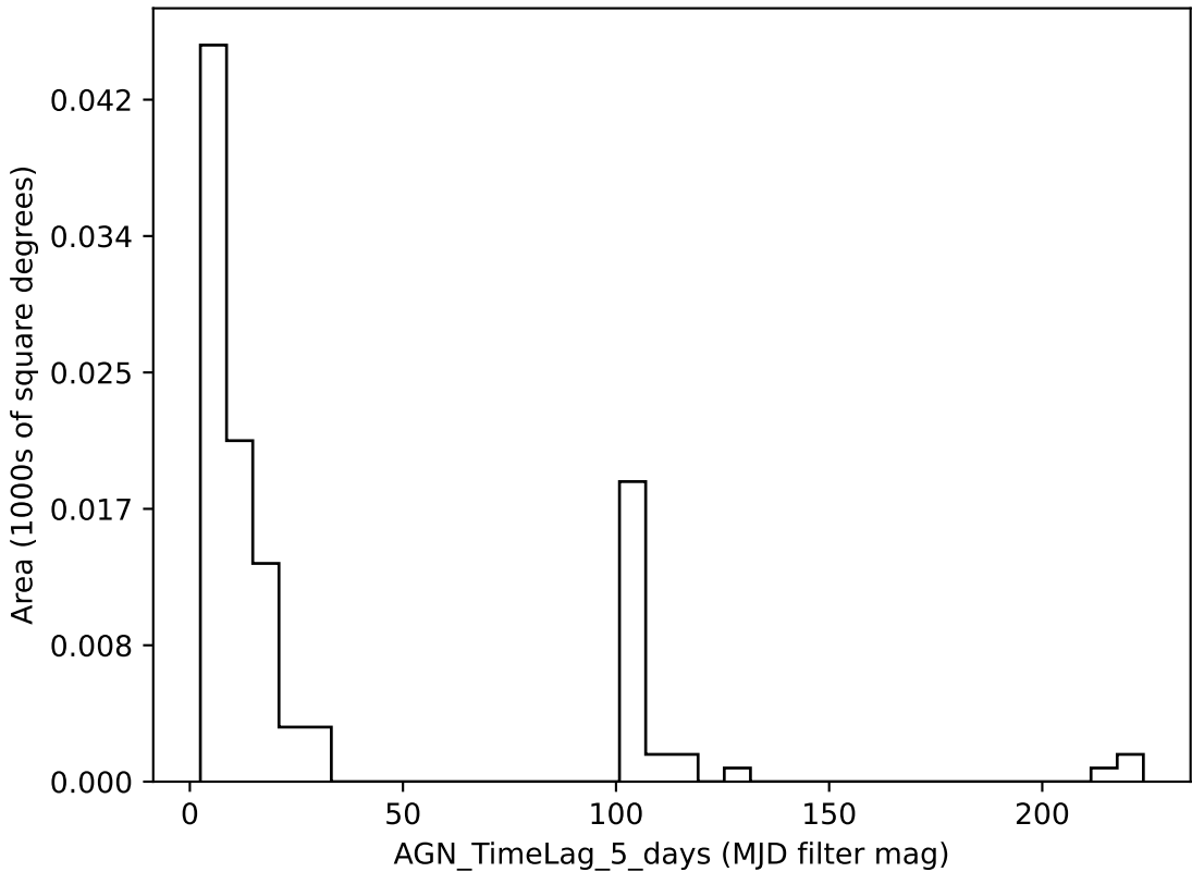
too_combined_s1.5_v3.4_10yrs all bands: AGN_TimeLag_5_days
