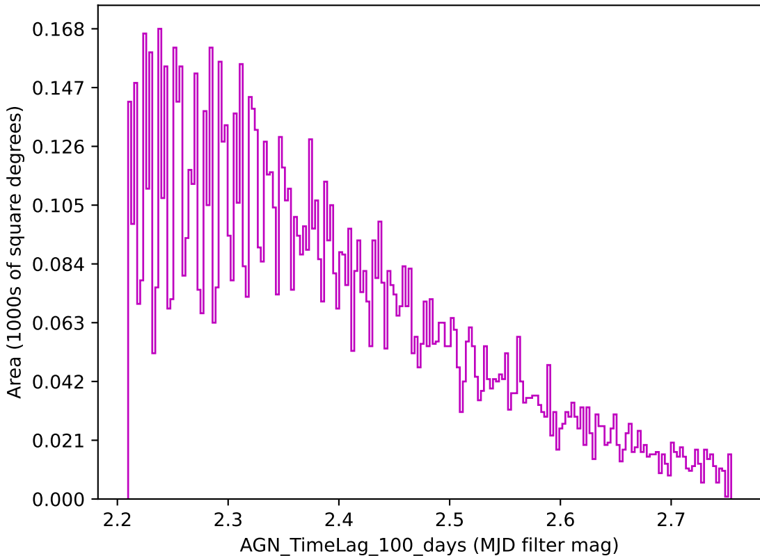
too_combined_s1.5_v3.4_10yrs z band: AGN_TimeLag_100_days
