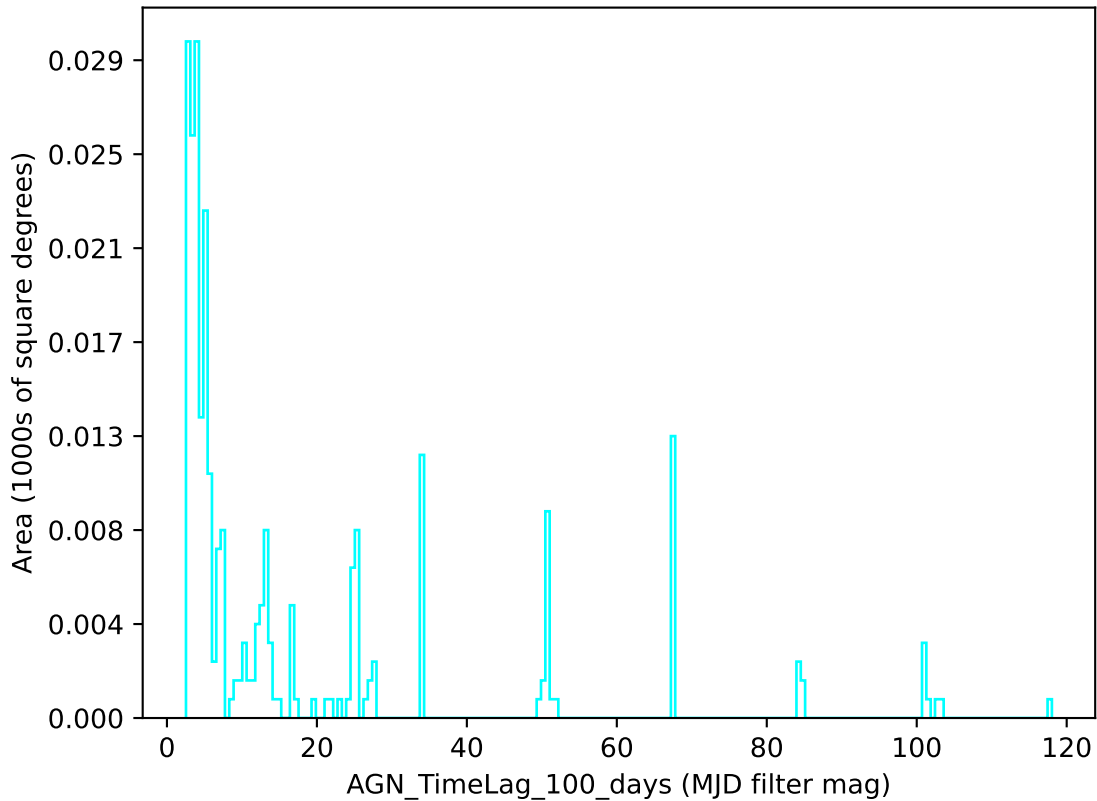
too_combined_s1.5_v3.4_10yrs u band: AGN_TimeLag_100_days
