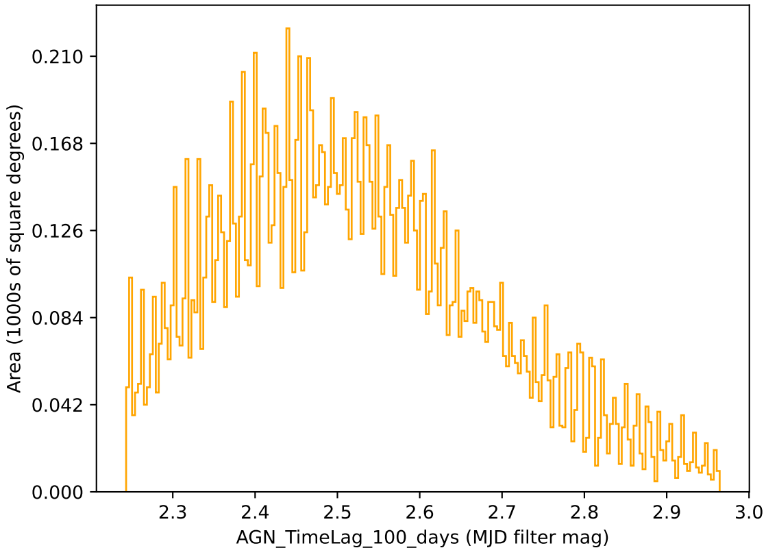
too_combined_s1.5_v3.4_10yrs r band: AGN_TimeLag_100_days
