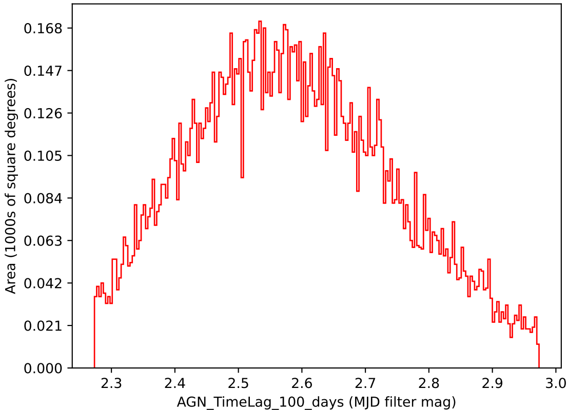
too_combined_s1.5_v3.4_10yrs i band: AGN_TimeLag_100_days
