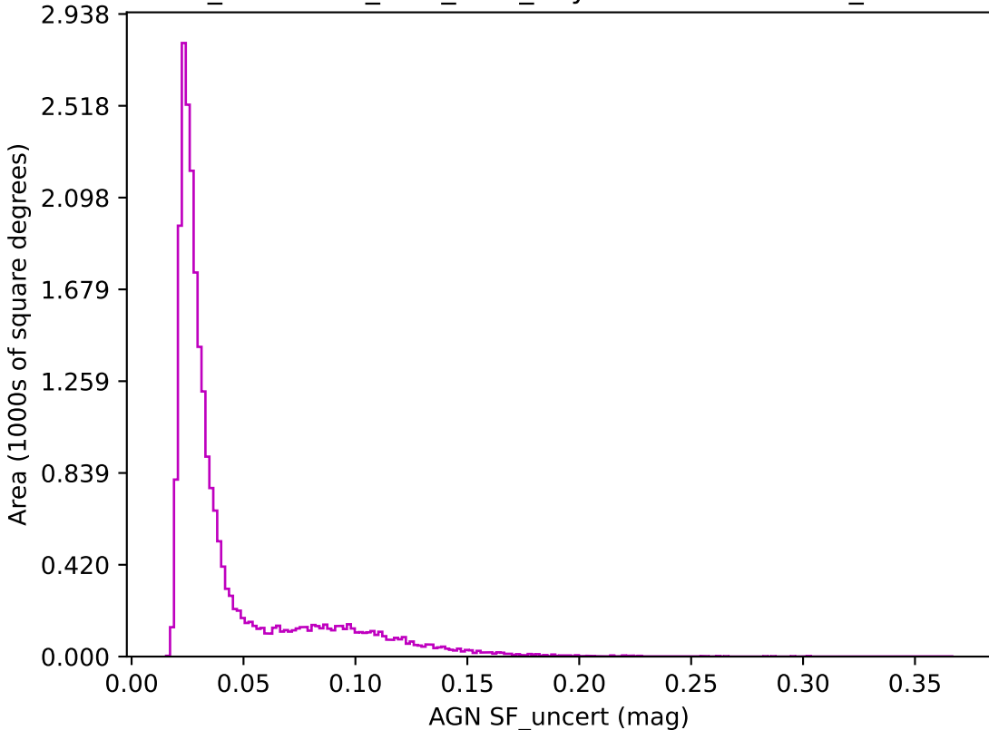
too_combined_s1.5_v3.4_10yrs z band: AGN SF_uncert
