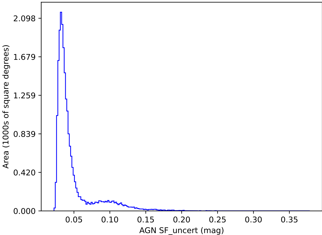
too_combined_s1.5_v3.4_10yrs y band: AGN SF_uncert
