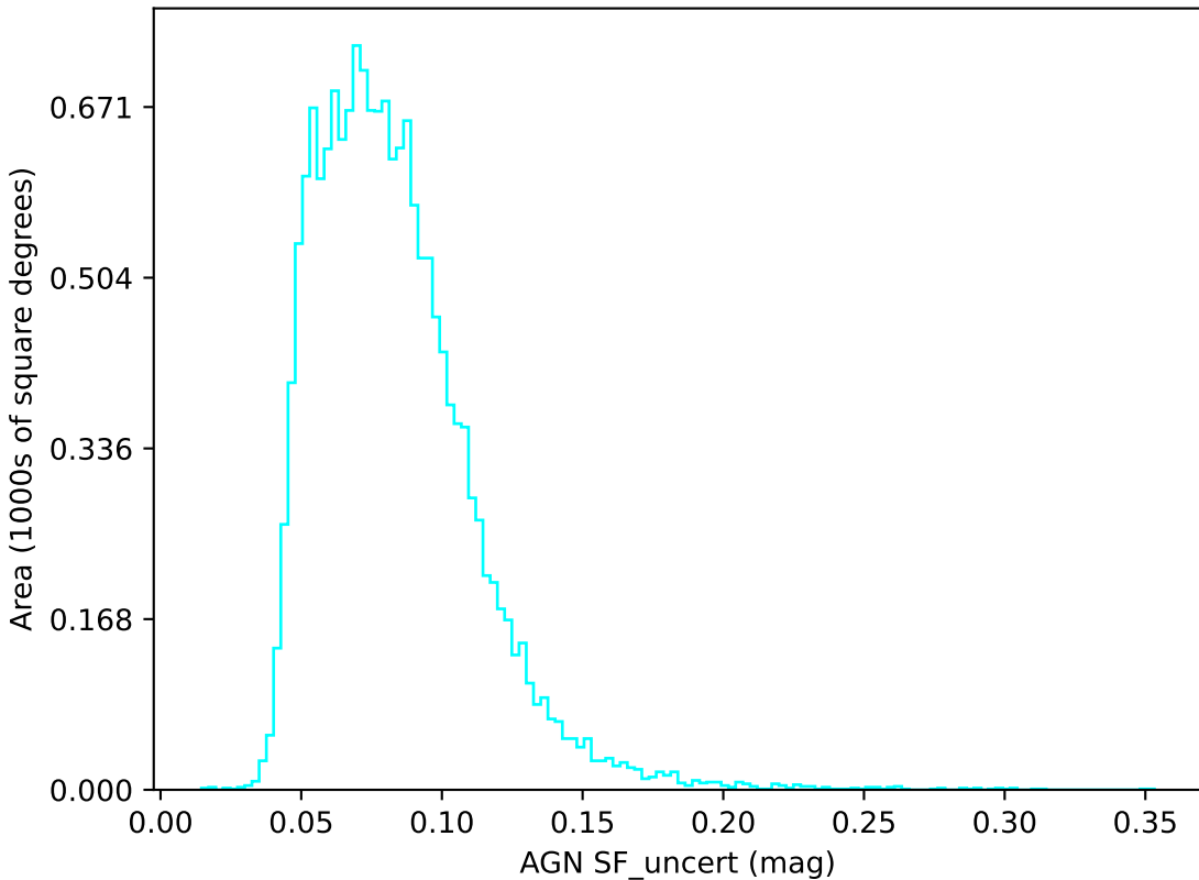
too_combined_s1.5_v3.4_10yrs u band: AGN SF_uncert
