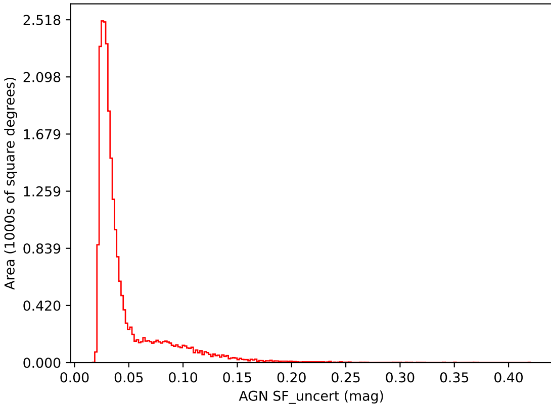
too_combined_s1.5_v3.4_10yrs i band: AGN SF_uncert
