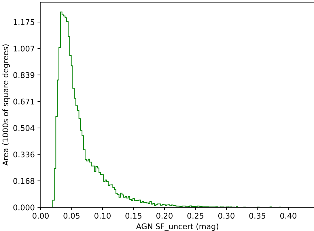
too_combined_s1.5_v3.4_10yrs g band: AGN SF_uncert
