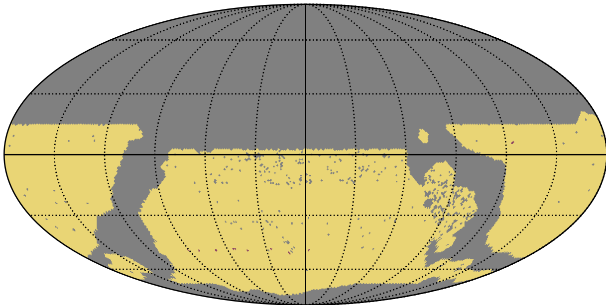
too_combined_s1.5_v3.4_10yrs WFD: RapidRevisits
