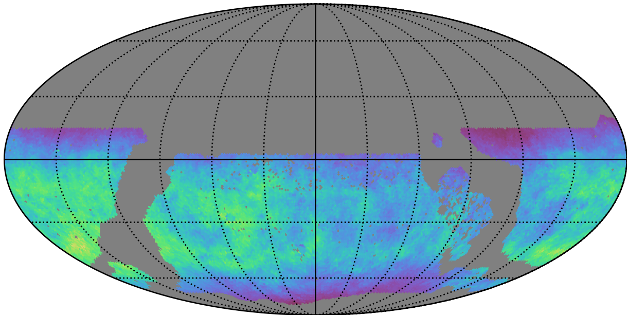
too_combined_s1.5_v3.4_10yrs WFD u band: Normalized Teff
