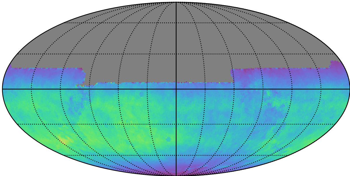
too_combined_s1.5_v3.4_10yrs All sky y band: Normalized Teff
