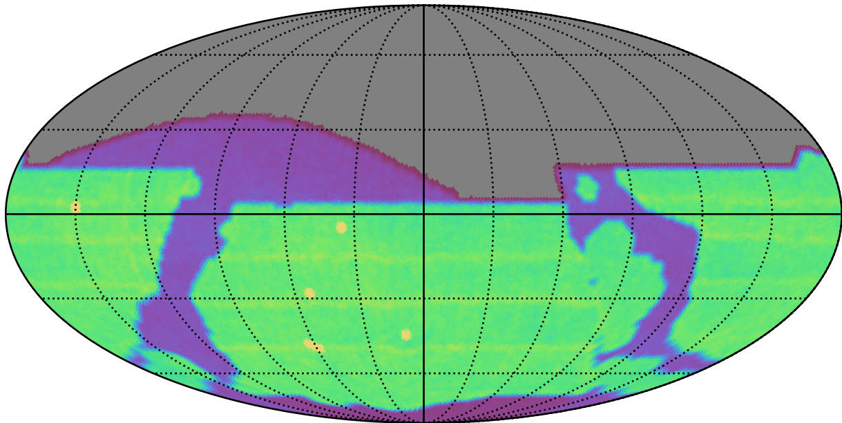
too_combined_s1.5_v3.4_10yrs All sky all bands: N Unique Nights
