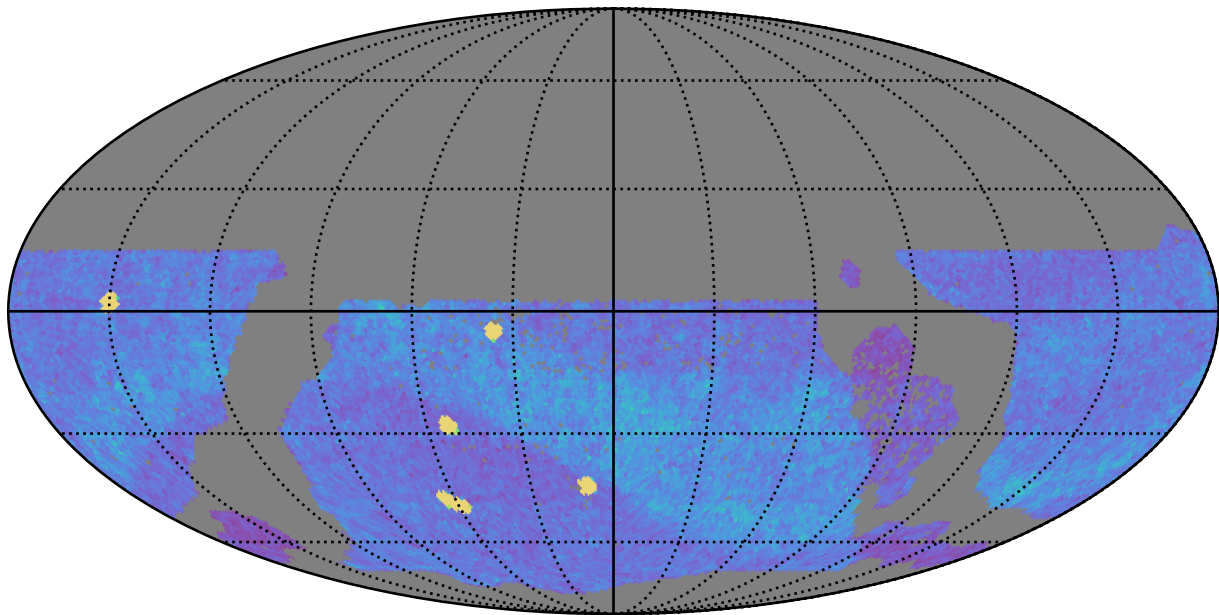
too_combined_s1.5_v3.4_10yrs WFD z band: NVisits
