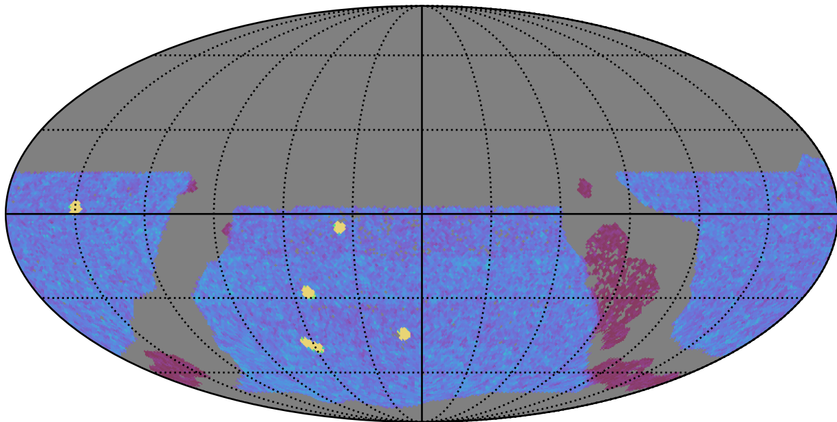
too_combined_s1.5_v3.4_10yrs WFD y band: NVisits
