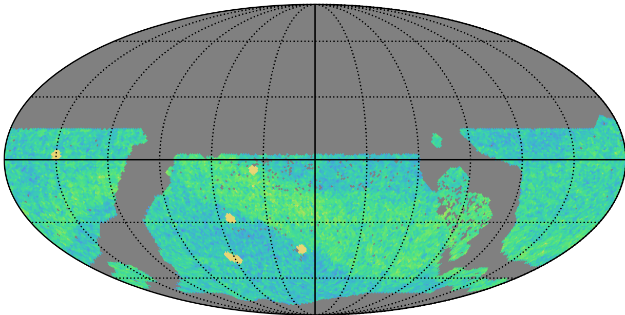
too_combined_s1.5_v3.4_10yrs WFD i band: NVisits
