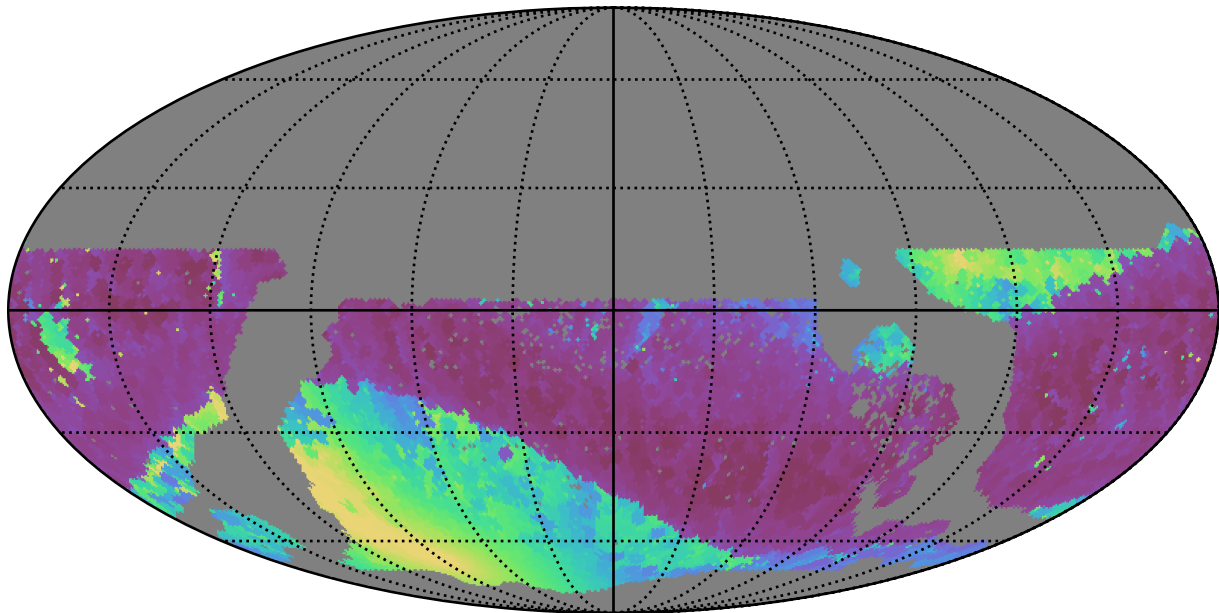
too_combined_s1.5_v3.4_10yrs WFD i band: Min solarElong
