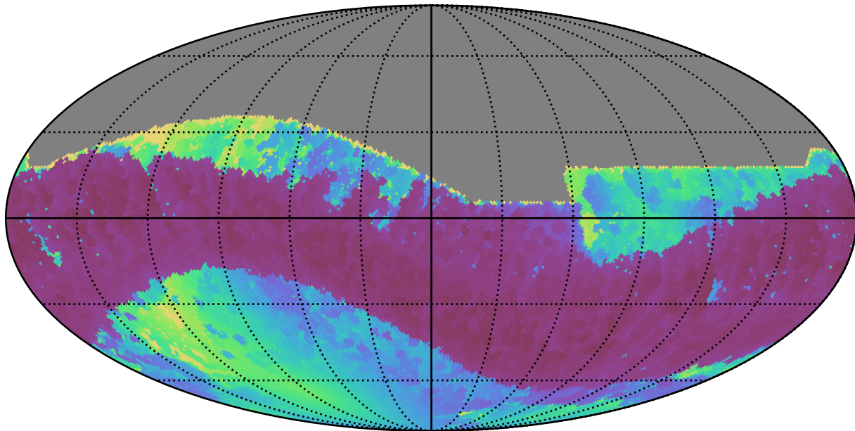
too_combined_s1.5_v3.4_10yrs All sky z band: Min solarElong
