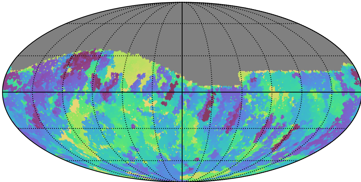
too_combined_s1.5_v3.4_10yrs Yr 1 r band: Min skyBrightness
