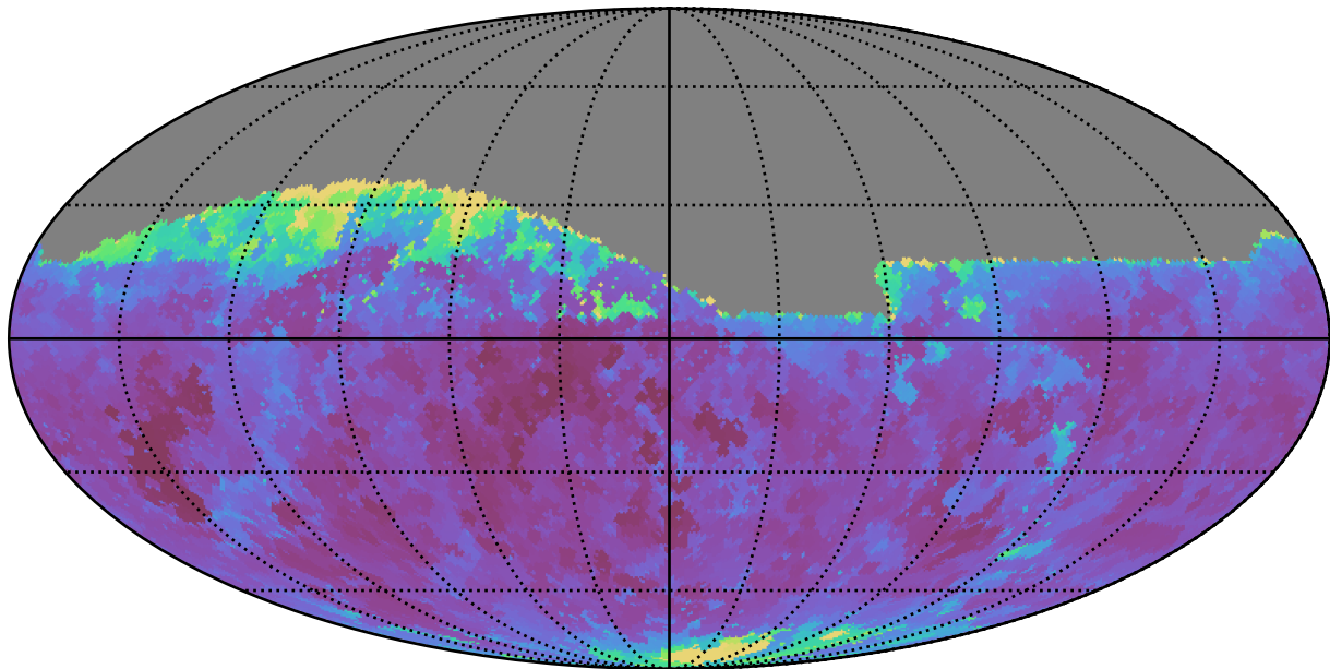
too_combined_s1.5_v3.4_10yrs Yr 1 i band: Min seeingGeom
