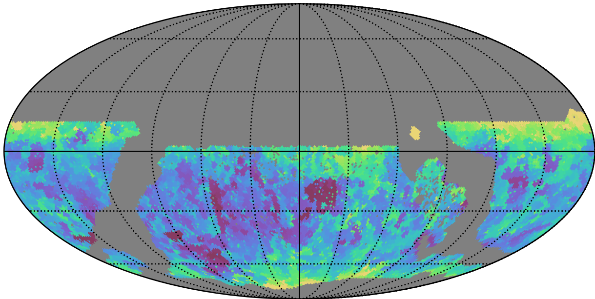
too_combined_s1.5_v3.4_10yrs WFD y band: Min seeingEff
