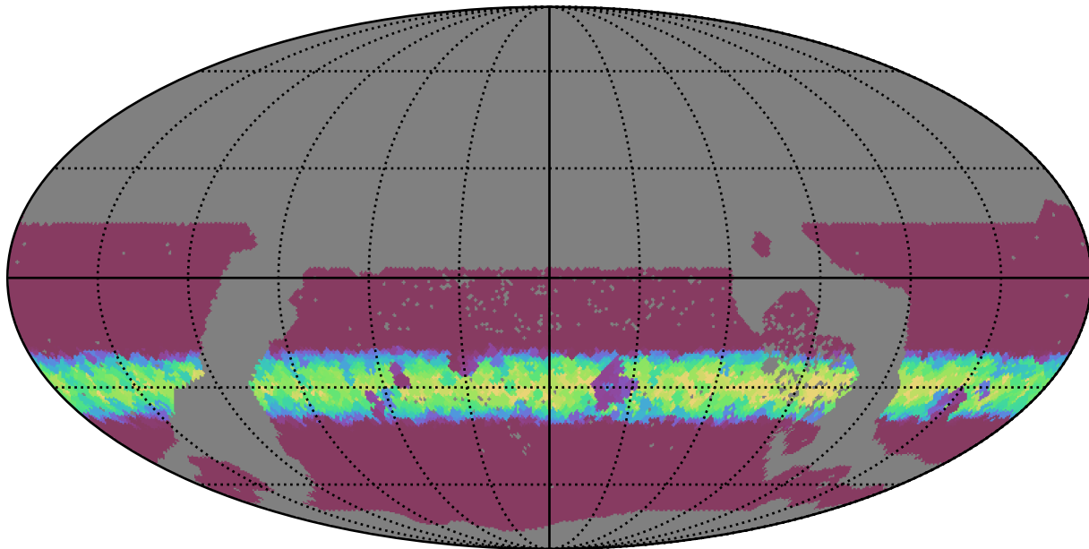
too_combined_s1.5_v3.4_10yrs WFD all bands: Min normairmass
