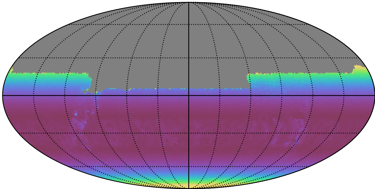
too_combined_s1.5_v3.4_10yrs All sky u band: Min airmass
