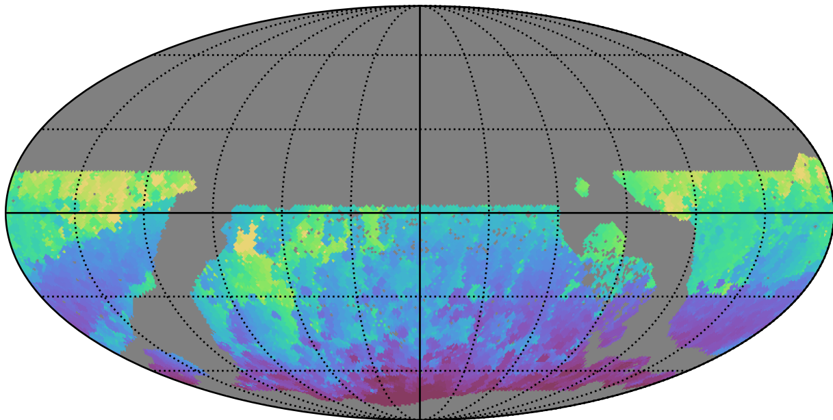
too_combined_s1.5_v3.4_10yrs WFD z band: Min HA
