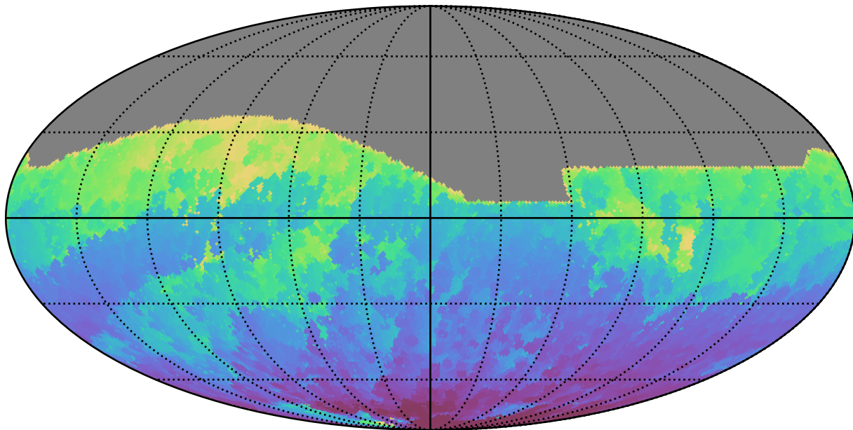
too_combined_s1.5_v3.4_10yrs All sky i band: Min HA
