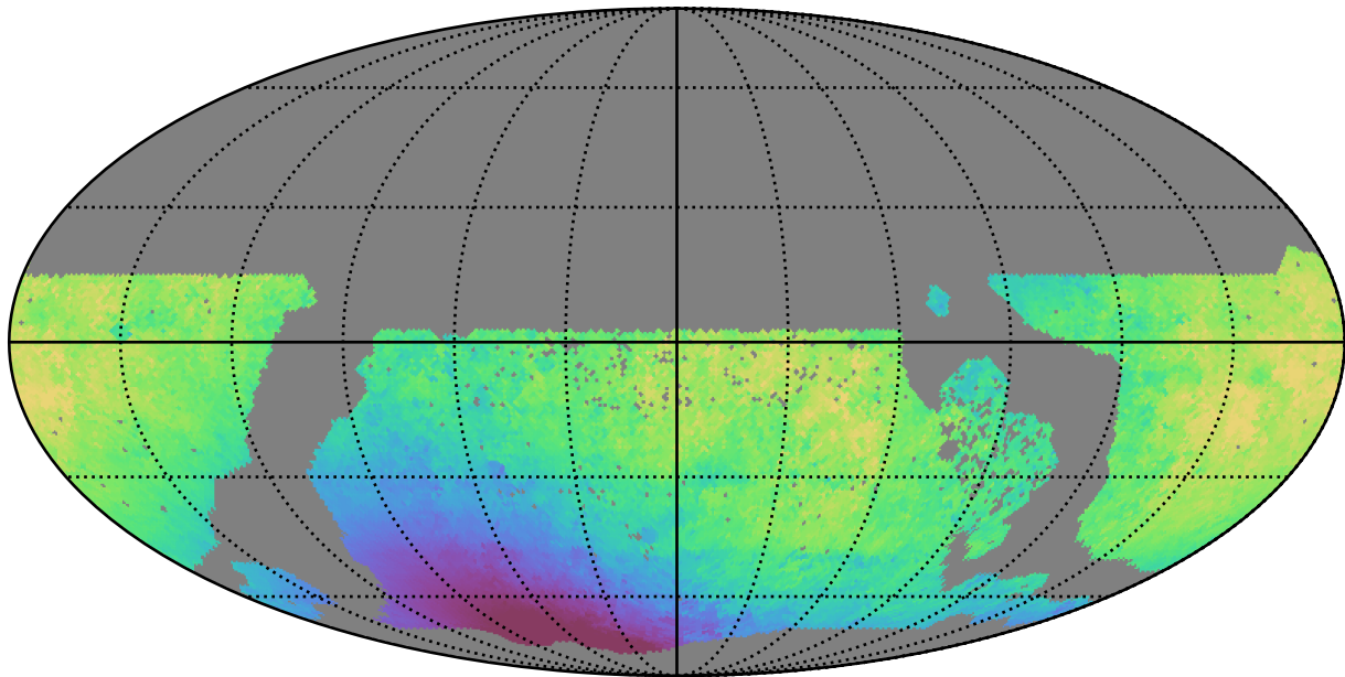
too_combined_s1.5_v3.4_10yrs WFD y band: Median solarElong
