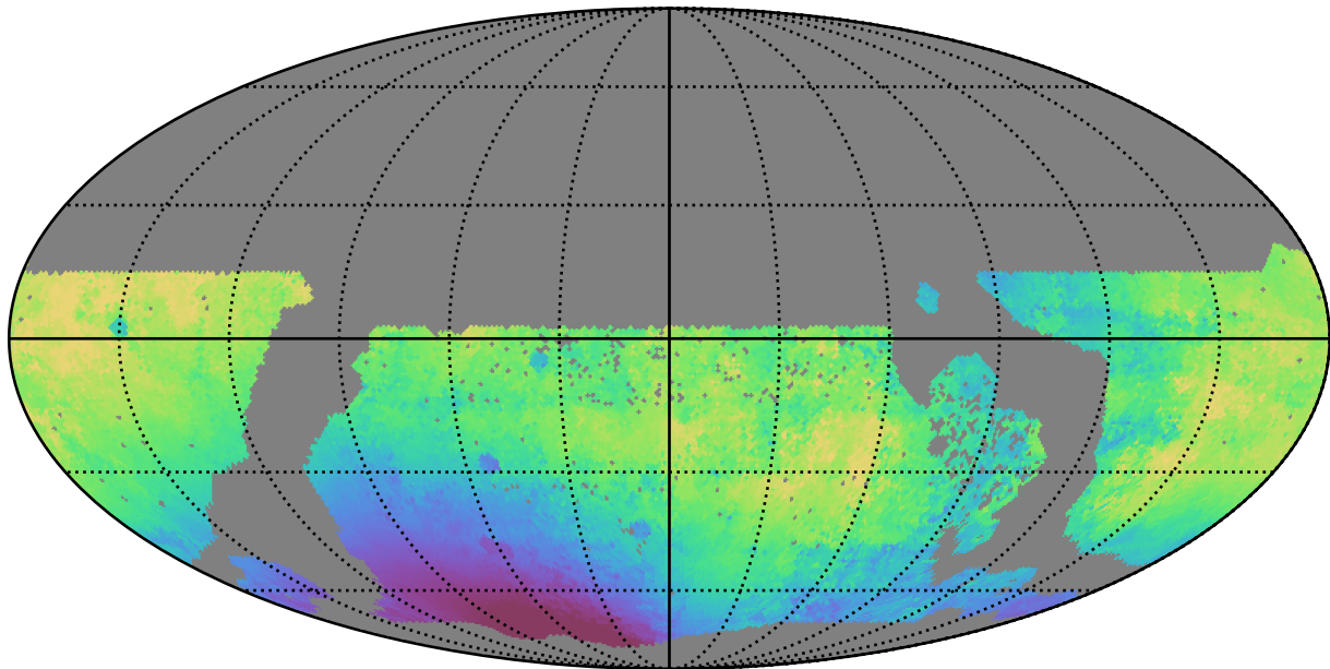
too_combined_s1.5_v3.4_10yrs WFD g band: Median solarElong
