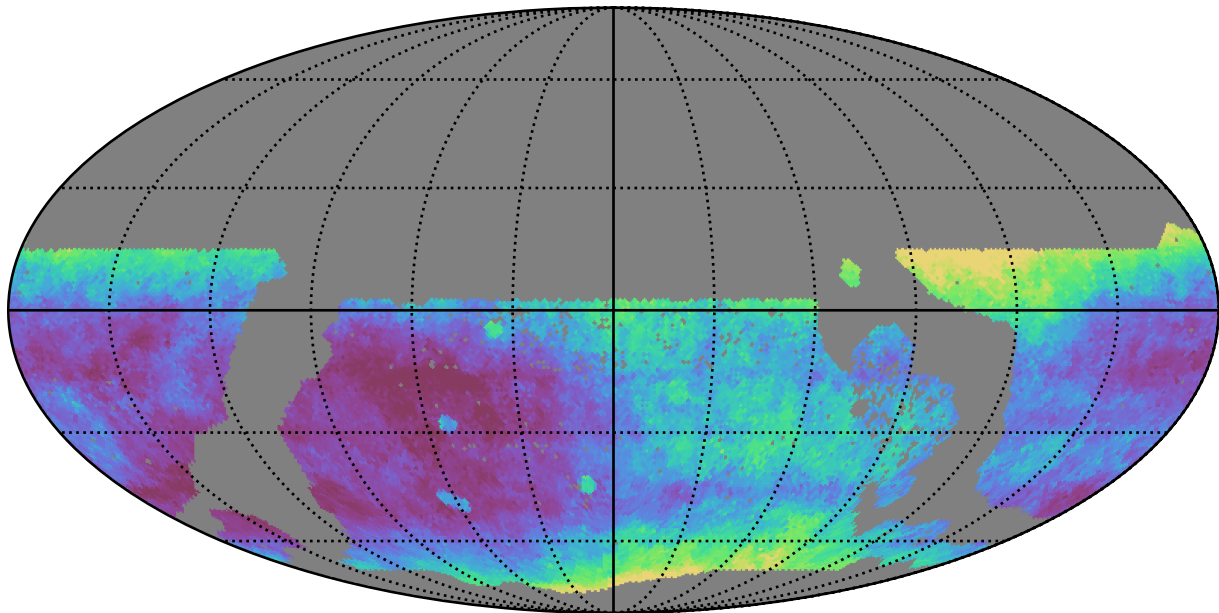
too_combined_s1.5_v3.4_10yrs WFD r band: Median seeingEff
