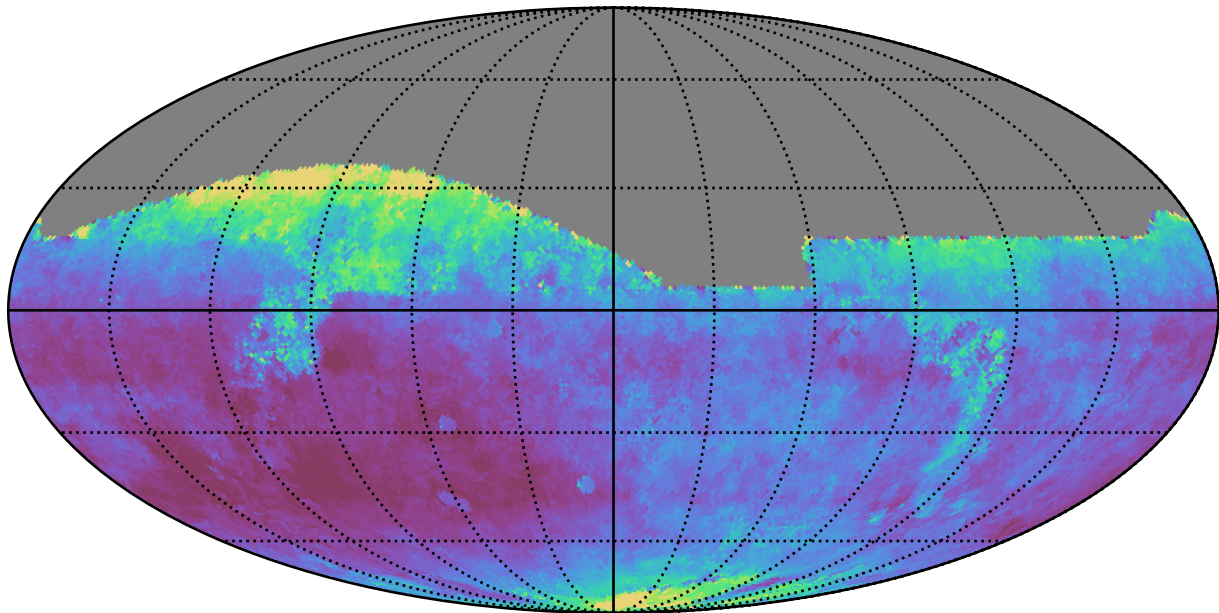
too_combined_s1.5_v3.4_10yrs All sky z band: Median seeingEff
