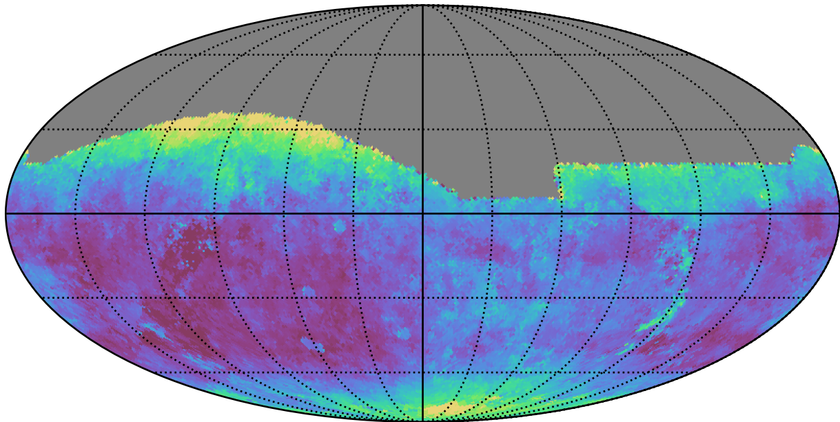
too_combined_s1.5_v3.4_10yrs All sky g band: Median seeingEff
