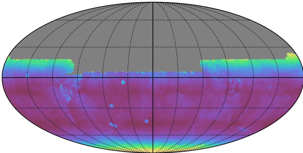
too_combined_s1.5_v3.4_10yrs All sky y band: Median airmass
