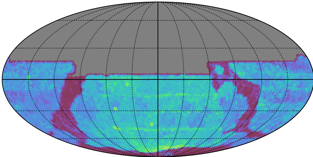
too_combined_s1.5_v3.4_10yrs All sky y band: Median Season Length
