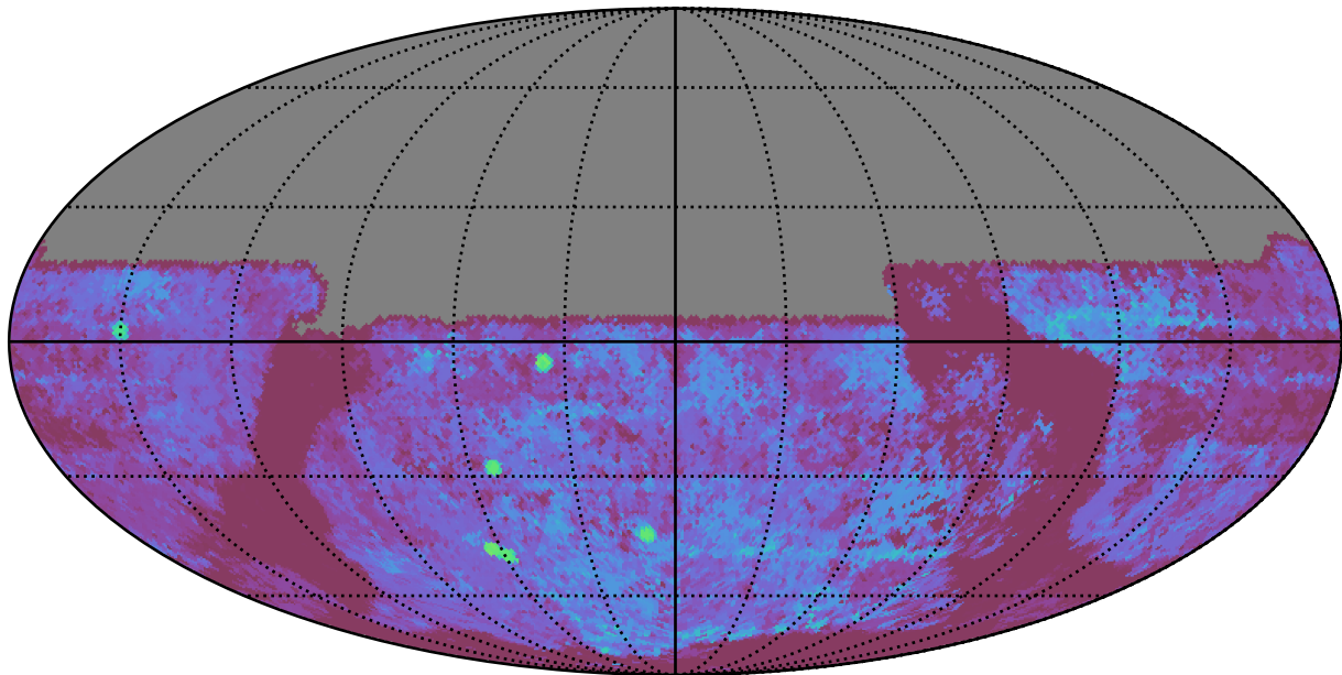
too_combined_s1.5_v3.4_10yrs All sky u band: Median Season Length
