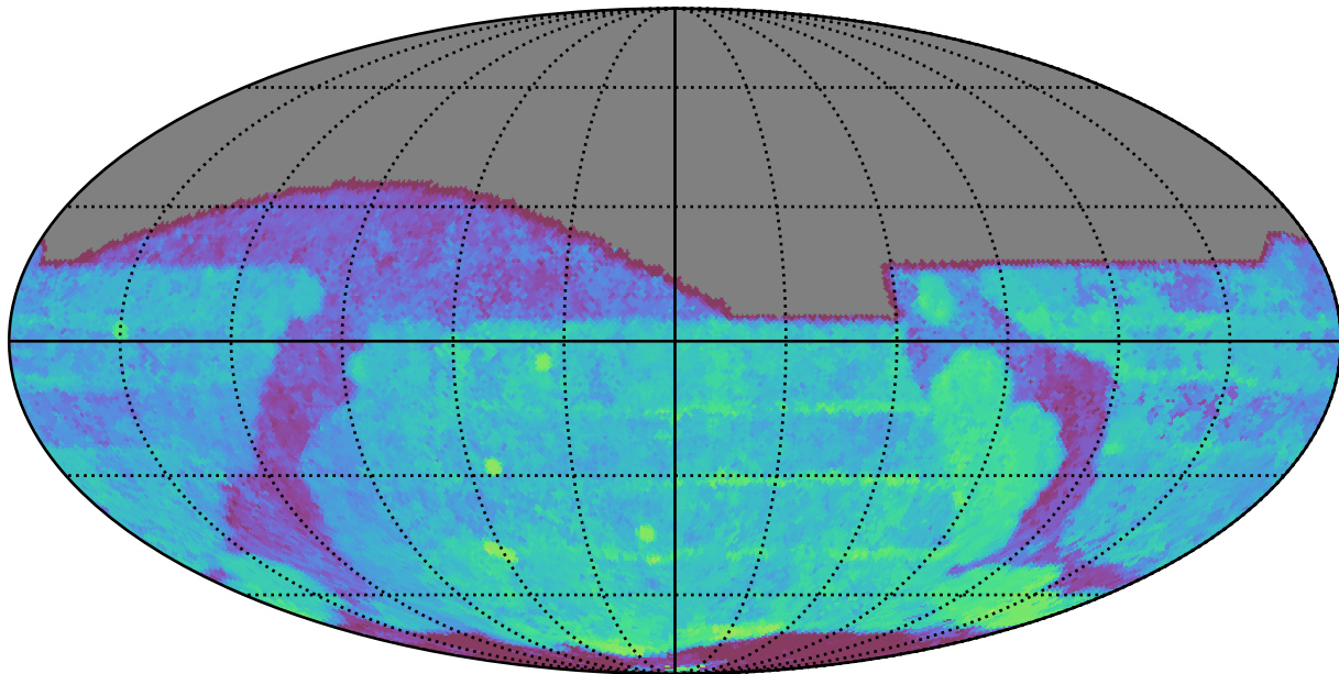
too_combined_s1.5_v3.4_10yrs All sky r band: Median Season Length
