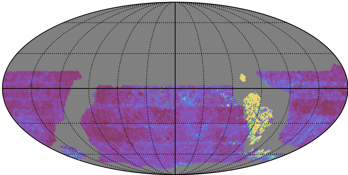
too_combined_s1.5_v3.4_10yrs WFD u band: Median Inter-Night Gap
