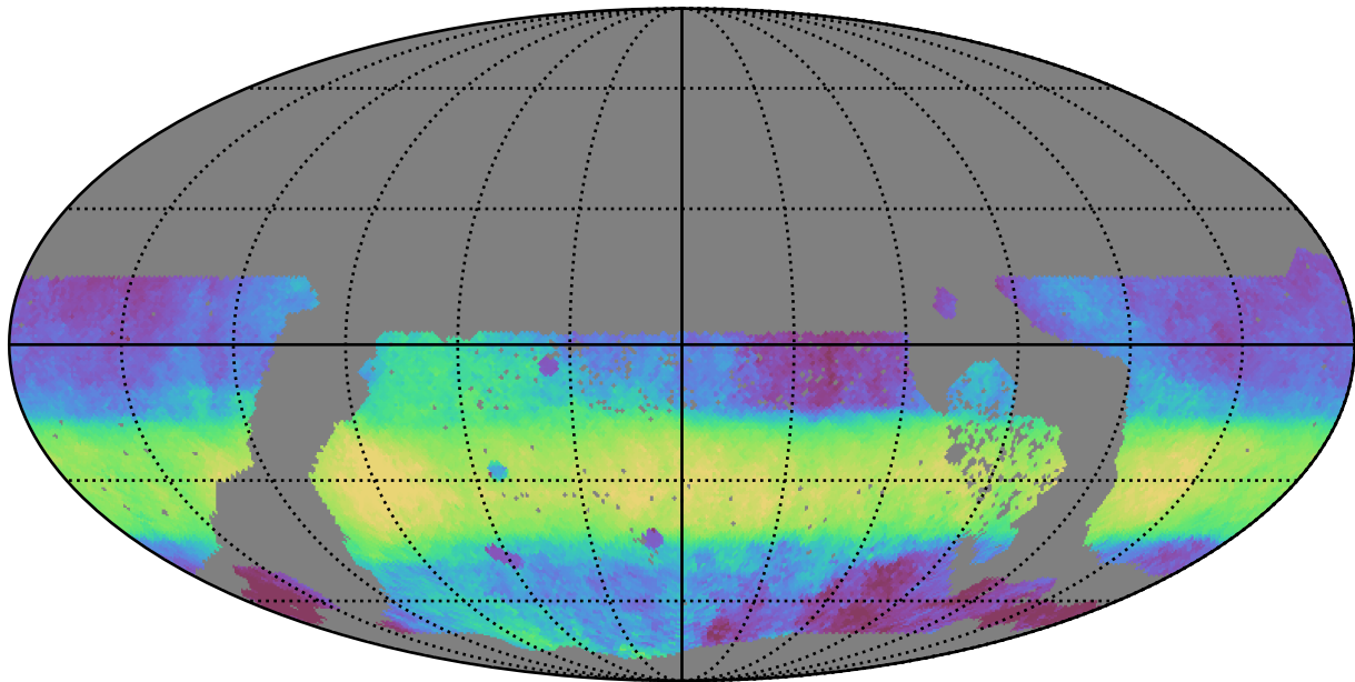
too_combined_s1.5_v3.4_10yrs WFD i band: Median HA
