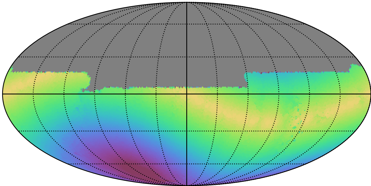
too_combined_s1.5_v3.4_10yrs All sky u band: Max solarElong
