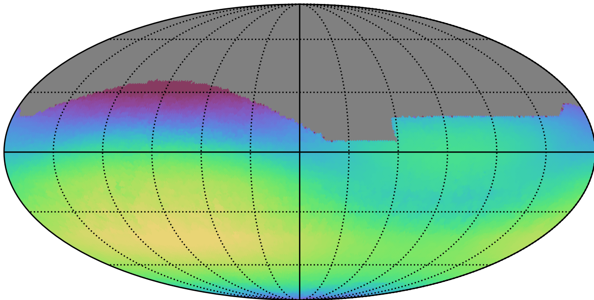
too_combined_s1.5_v3.4_10yrs All sky r band: Max skyBrightness
