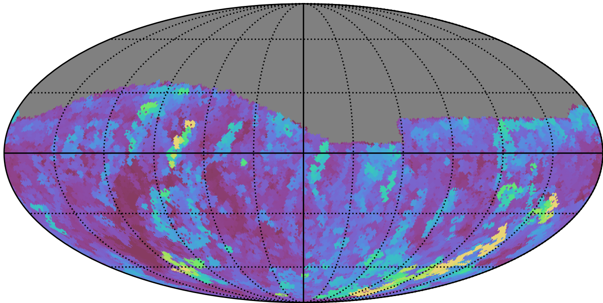
too_combined_s1.5_v3.4_10yrs Yr 1 r band: Max seeingEff
