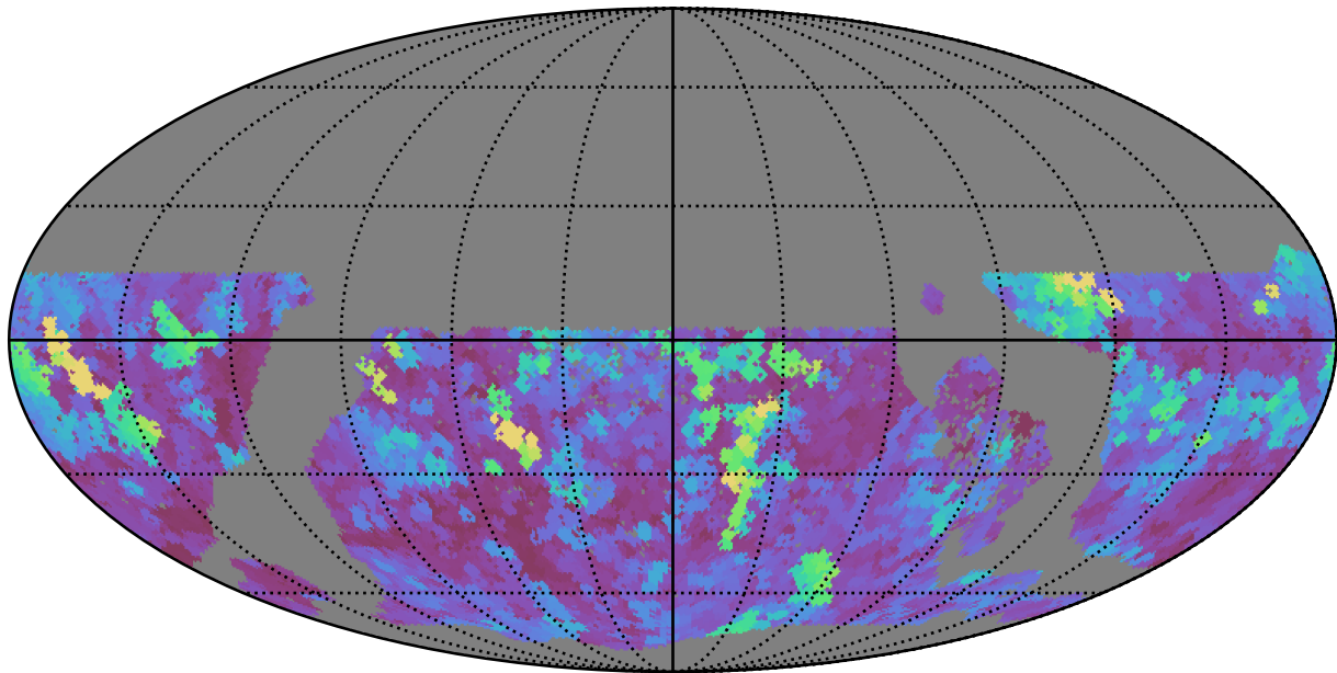
too_combined_s1.5_v3.4_10yrs WFD z band: Max seeingEff
