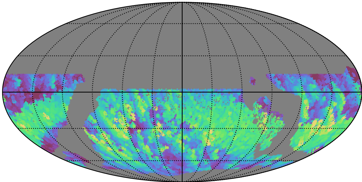
too_combined_s1.5_v3.4_10yrs WFD r band: Max normairmass
