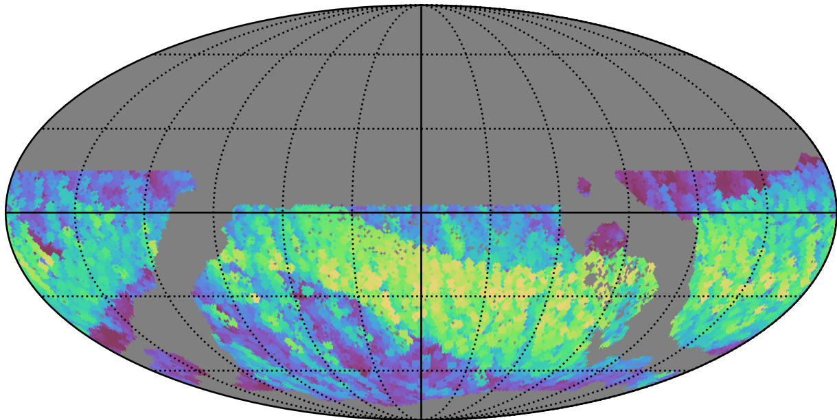
too_combined_s1.5_v3.4_10yrs WFD i band: Max normairmass
