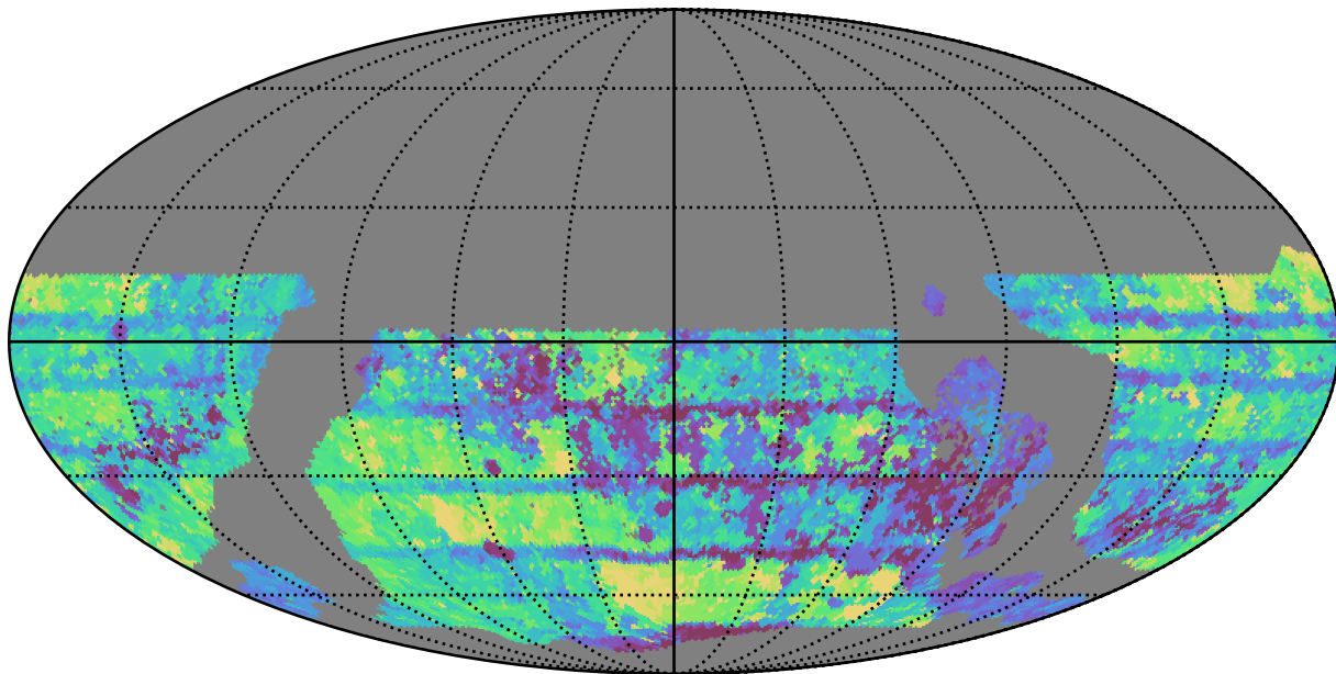
too_combined_s1.5_v3.4_10yrs WFD all bands: Max Inter-Night Gap
